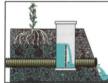
Controlled Subsurface Drainage (Std. 587 and Std. 554)
